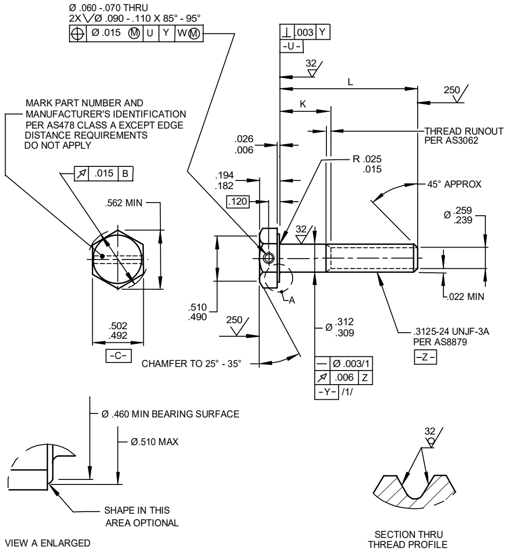
FIGURE 1 - BOLT
